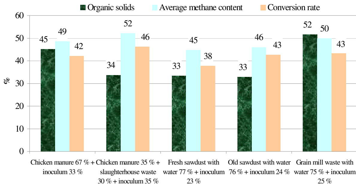
Fig. 3. Content of methane, organic solids and conversion rate from investigated waste
