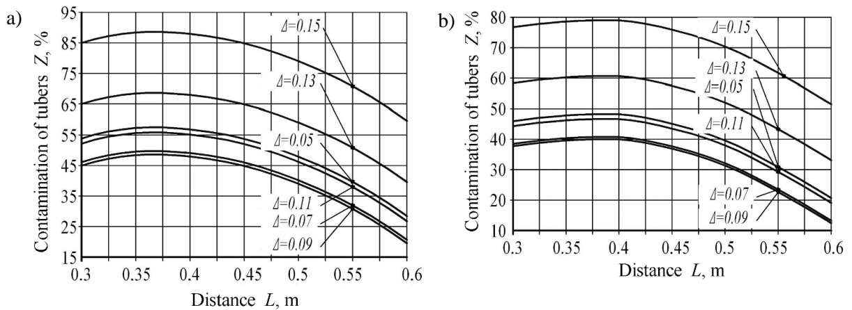
Fig. 3. Dependence of contamination of the tubers with impurities upon the distance between the drums and the distributor L , and the gap between the conveyor and the distributor \Delta :
