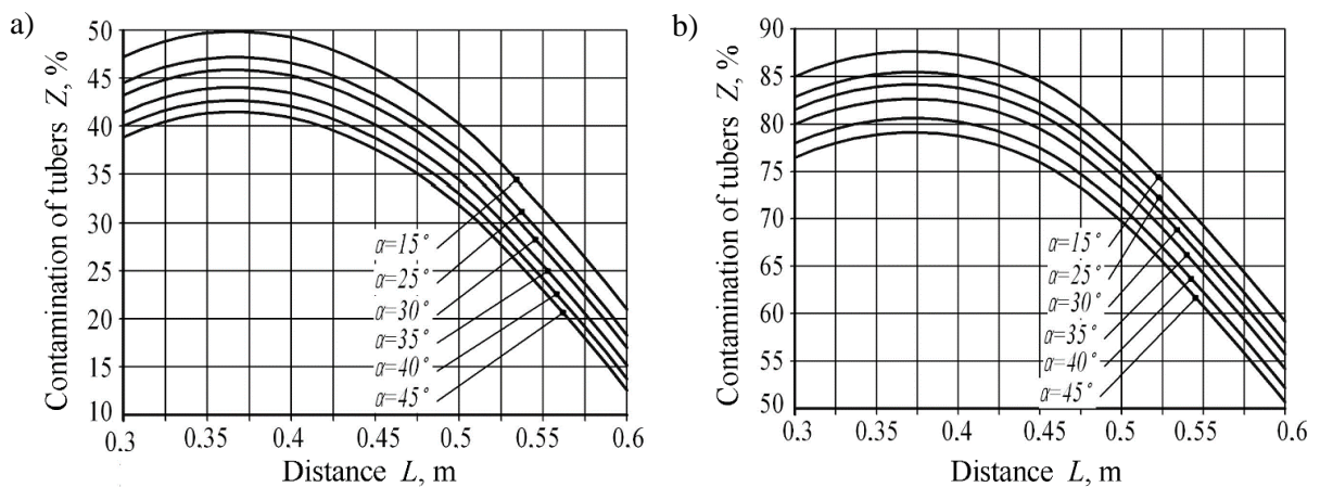
Fig. 4. Dependence of contamination of the tubers with impurities upon the distance between the drums and the distributor L , and the opening angle of the distributor wing \alpha :
